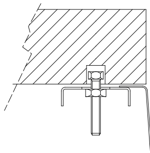
lateral section
